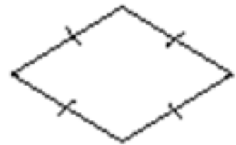
Rhombus (squashed square)
